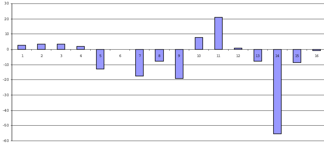
Figure 19: Ratios of shift factors to Sandow-Temple divided by outage shift factors to Bellso-Peters for selected busses.
