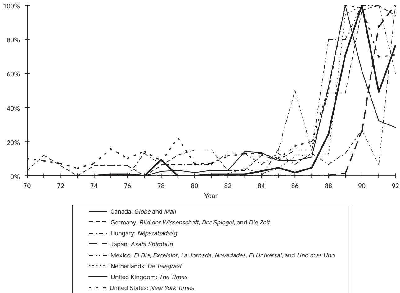
Figure 14.3 Country comparison of newspaper attention to climate change
