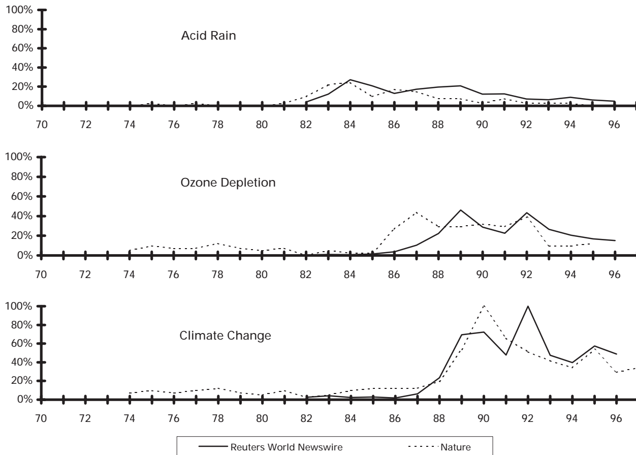
Figure 2.5 Attention to global atmospheric issues
