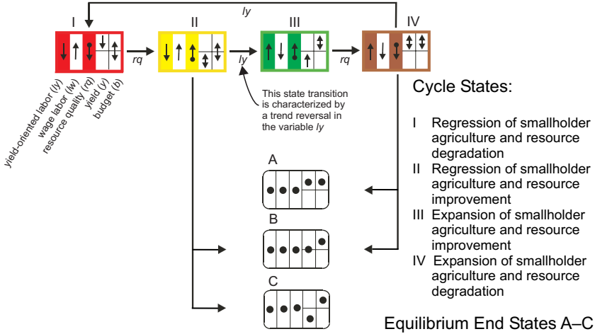
Figure 1.2 Symbolic dynamics of small agriculture in NE Brazil as a faithful projection to the five fundamental variables ly (yield-oriented labor), lw (wage-oriented labor), rq (resource quality), y (yield), and b (budget). The two sets of boxes represent cycle states (I–IV) and equilibrium end states (A–C), respectively, expressing magnitudes and trends of the fundamental variables by appropriate symbols. Dots indicate that the variable is constant over time, whereas trends are indicated by directed arrows. The crucial ly – rq trend combination is highlighted by color shading in the cycle state boxes. After Seitz et al., submitted.
