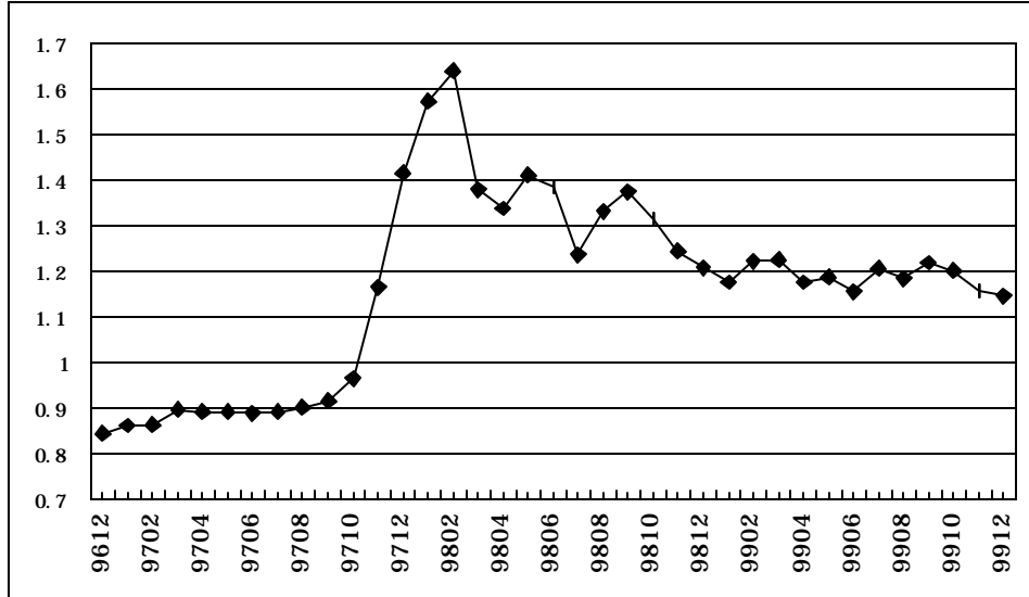
Figure 1. Korean Exchange Rate (1,000 Korean Won per US$)
