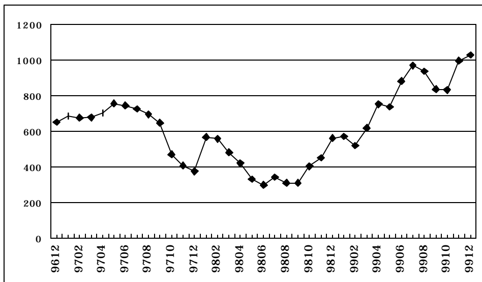
Figure 2. Korean Stock Price Index (KOSPI, in won, 1980 = 100)
